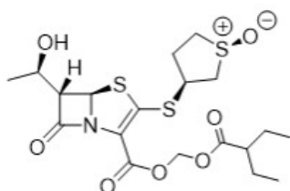
Figure 1. Sulopenem Etzadroxil Chemical Structure and Formula
