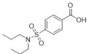
Figure 2. Probenecid Chemical Structure and Formula
